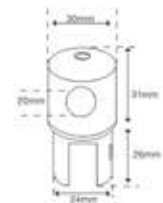
KSKH-05 Rod to Glass Connector
