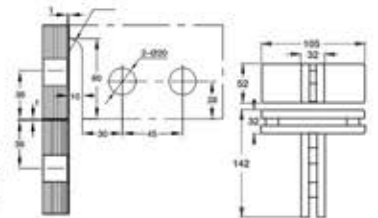
Cut Out Details
