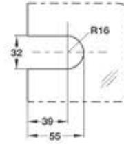
Cut Out Details
