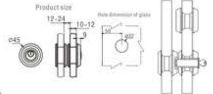
KSL-30L Sliding Door Lock (Glass to Glass)
