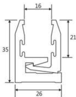
KGP-22 Glazing Profile
