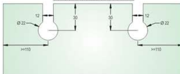
CUTOUT DETAILS OF SSL-44-A2
