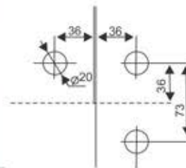
Cut Out Details
