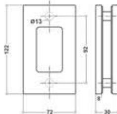
KSL-HN 40 Rectangle Handle
