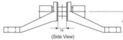
KSF-A2 Two Way Spider with Fin
