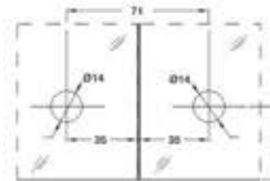
Cut Out Details
