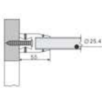
KSL-33-TH-WL Wall to Rod Holder
