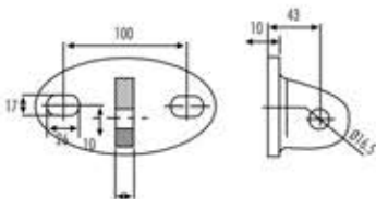
KCF-03 Wall Connector
