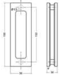
KSL-HN 10 Rectangle Handle
