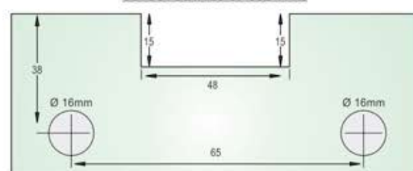
CUTOUT DETAILS OF SSL-44-R8
