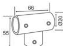
KSKH-04 Rod to Rod T Connector
