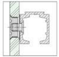
KSL-06 Glass to Track Clamp
