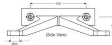
KSF-A44 Two Way Spider with Fin (Wall Mounted)
