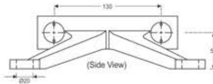
KSF-A4 Four Way Spider with Fin
